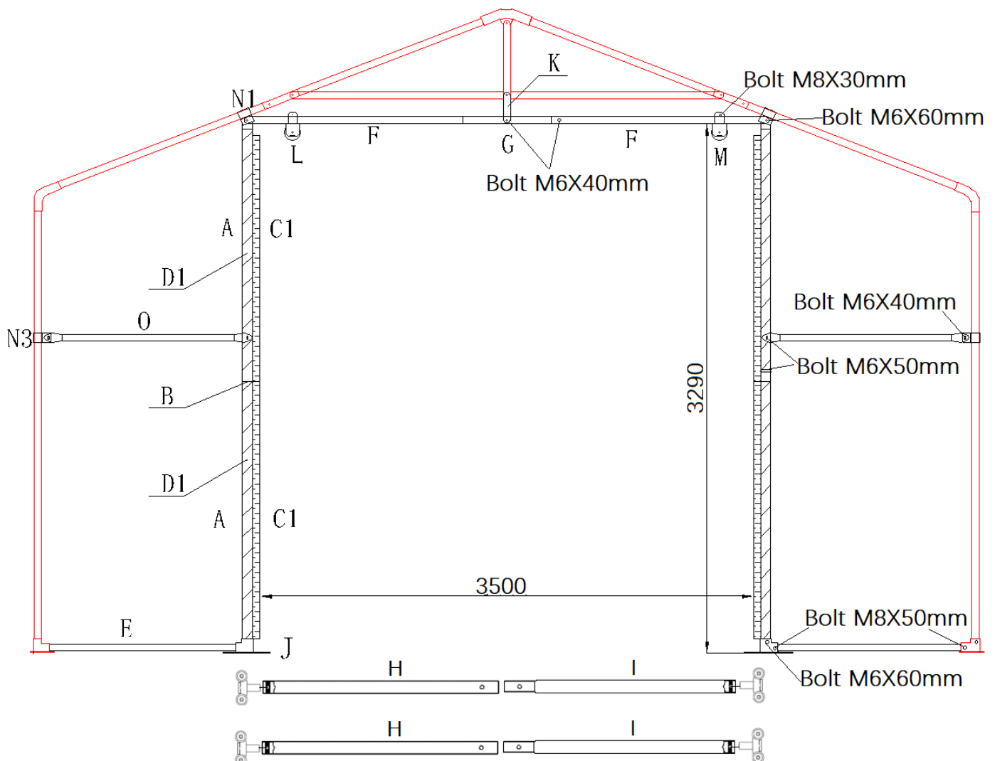
Frame of Pull-up End wall
